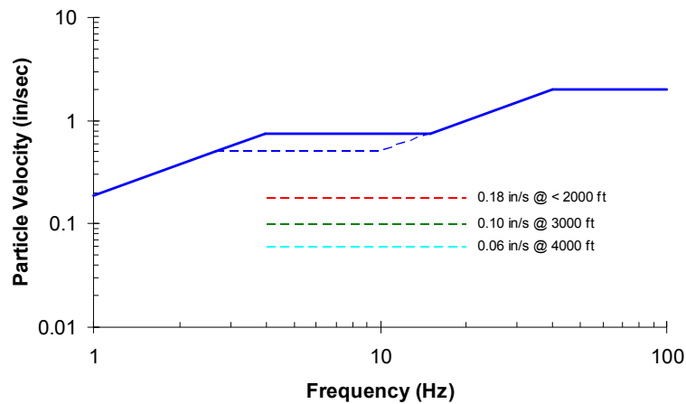
Figure 3. RI 8507 Safe Blasting Levels and expected vibration levels from blasting at the New Shine Quarry, WA (for distances less than 2,000 feet, the use of 2 decks per hole has been assumed).
