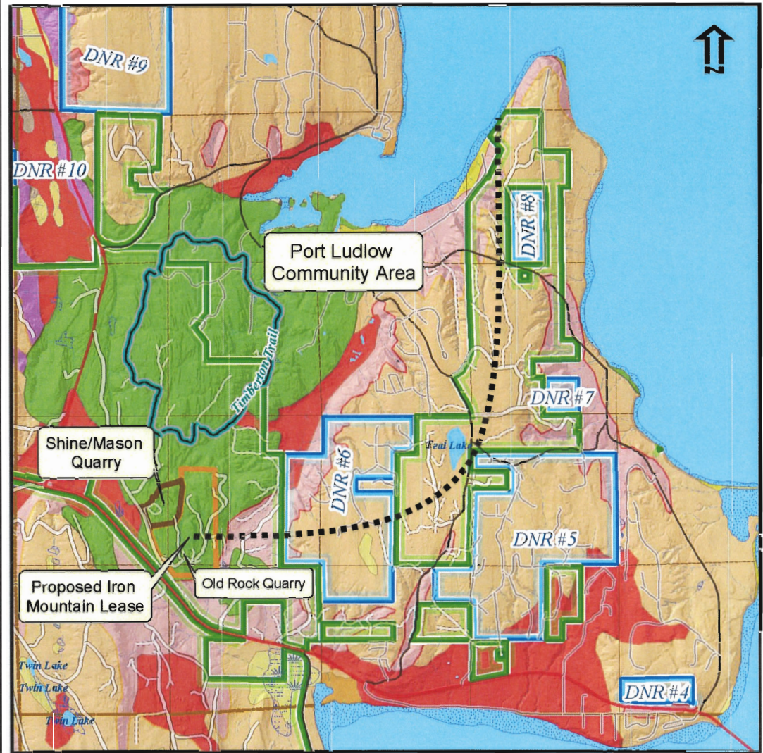
Exhibit 2 - Underlying Geology
